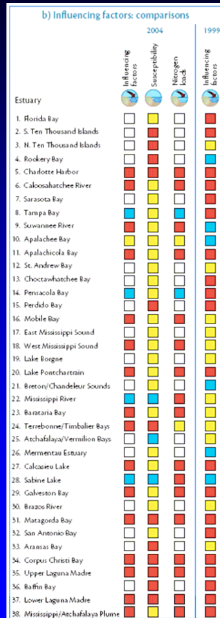
Figure 4.14. (a) Map of influencing factors ratings and (b) ratings of components of influencing factors and 1999 ratings in the Gulf of Mexico region.
