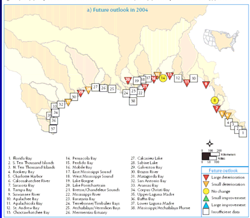
Figure 4.16. (a) Map of Gulf of Mexico future outlook in 2004 and (b) in comparison with the 1999 future outlook
