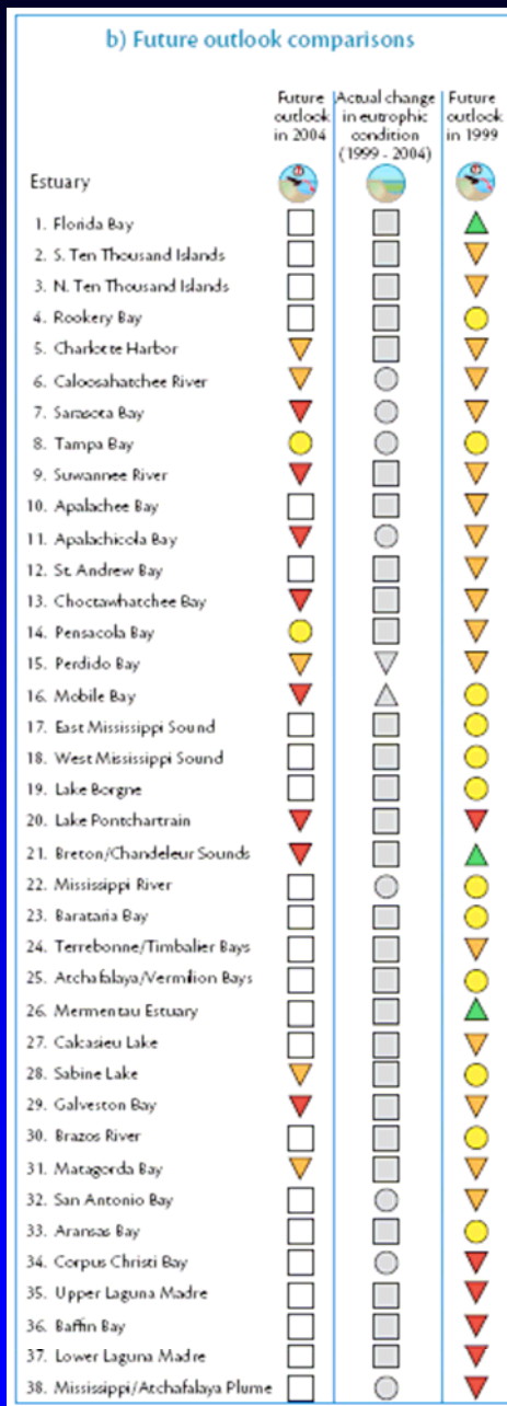
Figure 4.16. (a) Map of Gulf of Mexico future outlook in 2004 and (b) in comparison with the 1999 future outlook
