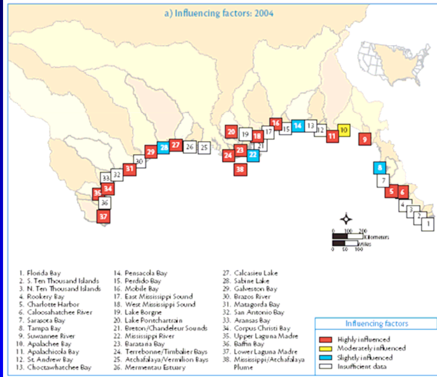
Figure 4.14. (a) Map of influencing factors ratings and (b) ratings of components of influencing factors and 1999 ratings in the Gulf of Mexico region.
