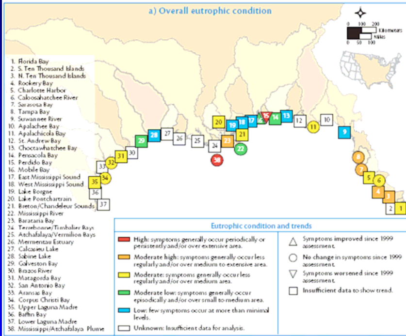
Figure 4.15. a) Map of overall eutrophic condition (OEC) and (b) the combination of individual eutrophic symptoms which constitute OEC ratings in the Gulf of Mexico region.
